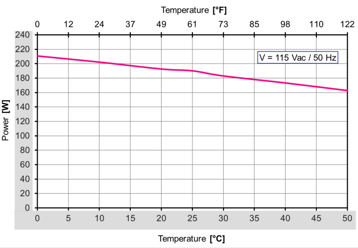
Power-Temperature
