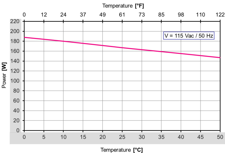
Power-Temperature
