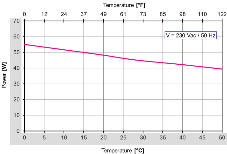
Power-Temperature
