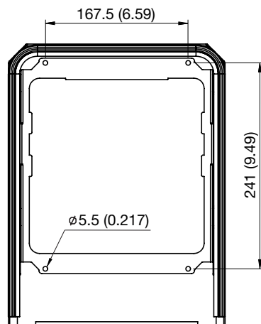
Mounting cut-out mm (in)
