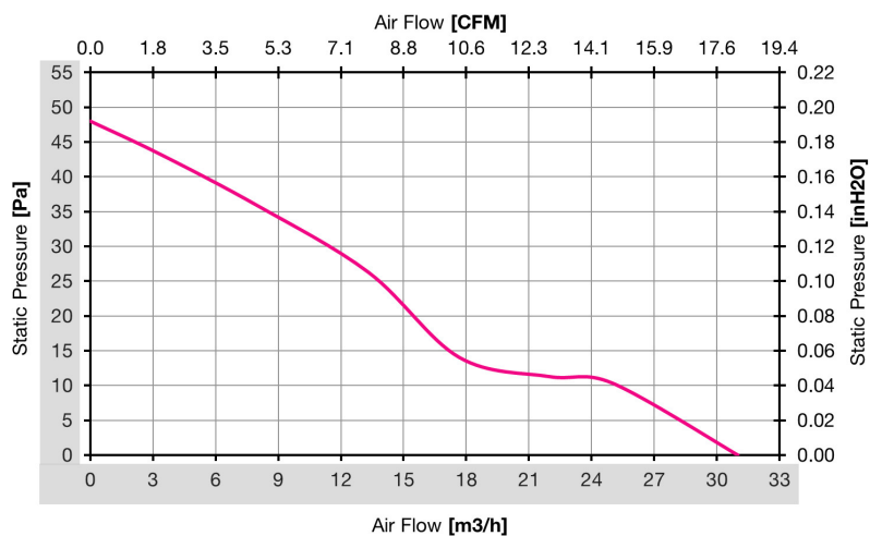
Air Performance
